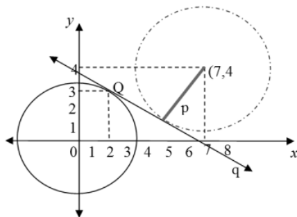
Figure 1. Position of both circles L_1 and L_2 in one Cartesian coordinate system
